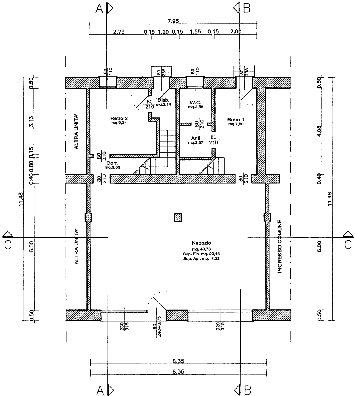
Piano Terra scala 1:100
